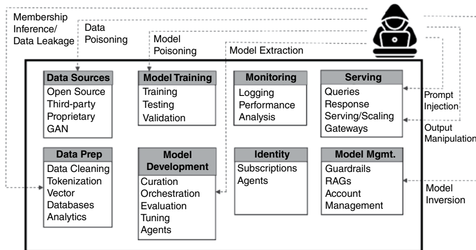
Figure 4.1 Common attack patterns targeting each stage of the AI development framework
