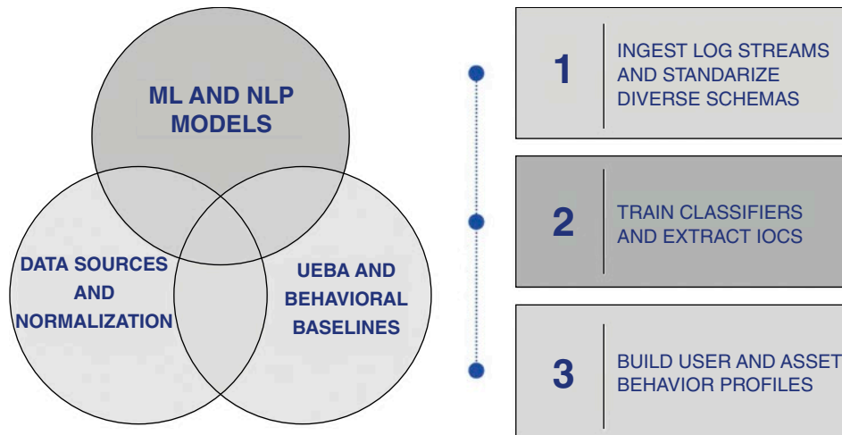
FIGURE 10.3. MetroBank deployment architecture. Normalized data feeds, ML/NLP classifiers, and UEBA profiles form the analytical core that supports correlation, triage, and investigation.
