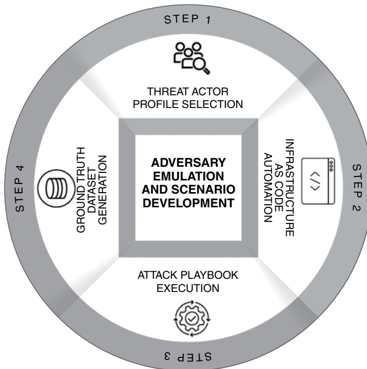
FIGURE 3.7. Adversary emulation and scenario development cycle. Steps 1–4 correspond directly to the numbered discussion above: threat actor profile selection, IaC automation, attack playbook execution, and ground-truth dataset generation.
