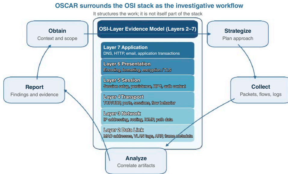
FIGURE 2.2. OSCAR workflow surrounding the OSI-layer evidence model.
