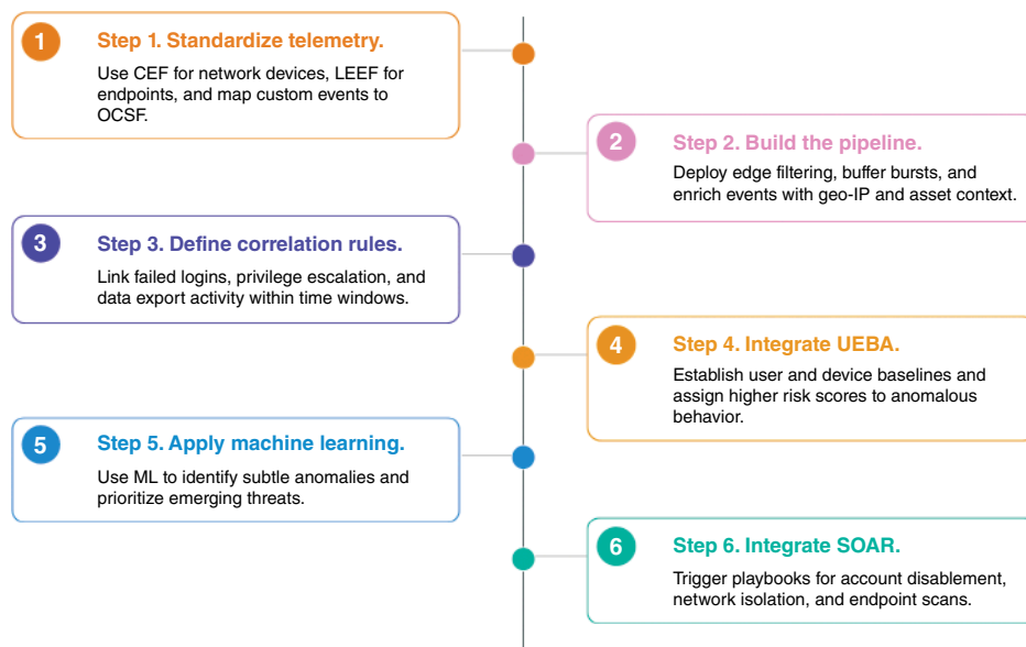
FIGURE 8.3. AFS implemented behavioral SIEM in six stages: standardize telemetry, build the pipeline, define correlation rules, integrate UEBA, apply machine learning, and automate response with SOAR.
