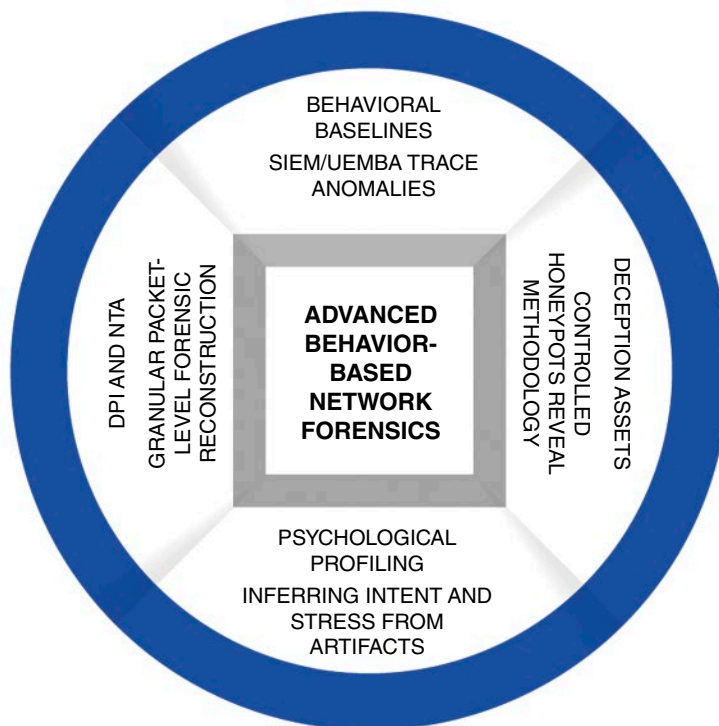
FIGURE 6.1. Core components of advanced behavior-based network forensics: behavioral baselines identify anomalies, deception assets generate high-confidence forensic clues, DPI/NTA reconstruct network activity, and psychological profiling adds human-context analysis to technical evidence.
