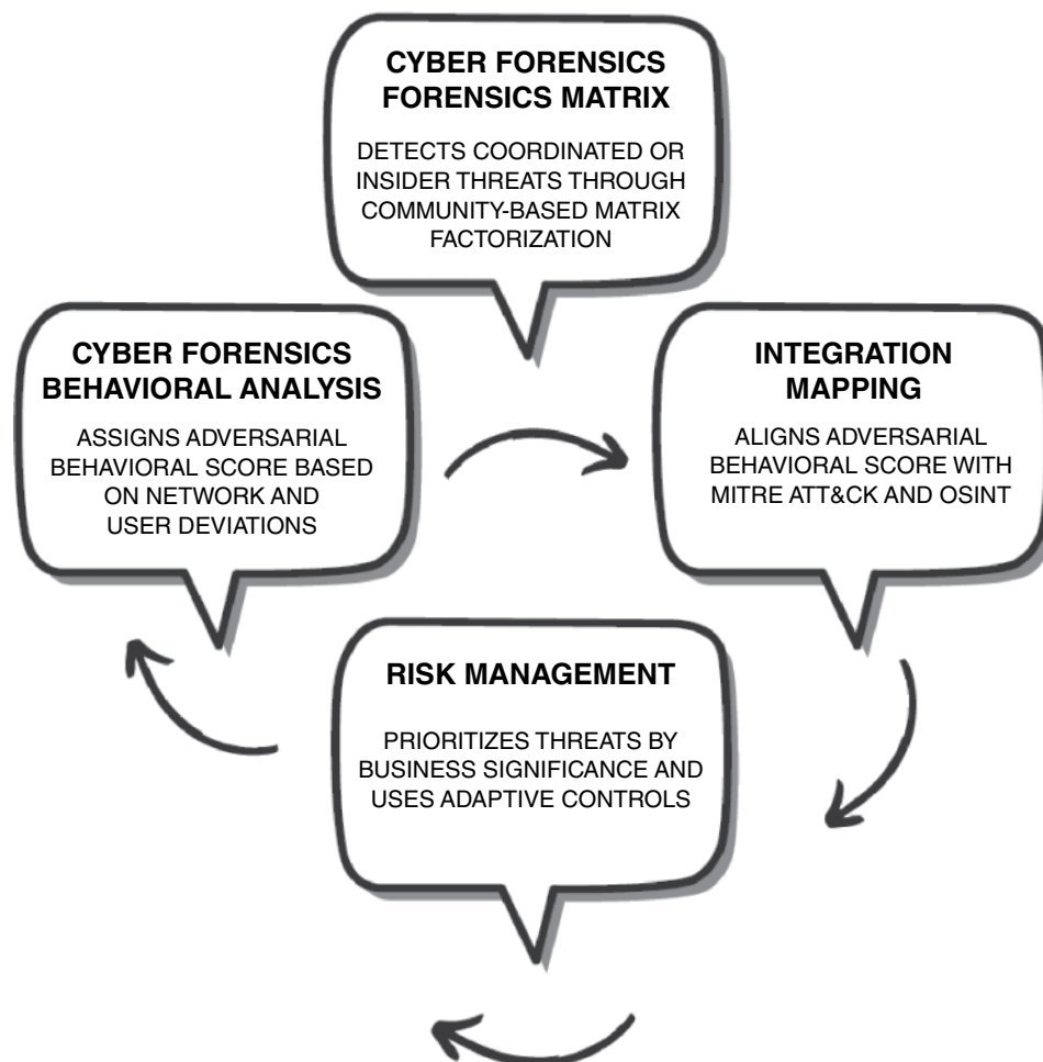
FIGURE 12.3. Cohesive and synergistic response model. CFBA produces ABS from user and network deviations; CBFM uses CBFM to identify anomalous communities; integration mapping aligns those indicators with MITRE ATT&CK and OSINT; and risk management converts the results into prioritization and adaptive controls.
