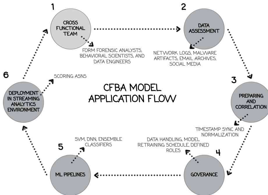
FIGURE 5.2. CFBA application flow. The workflow shows how a cross-functional team combines data assessment, preparation and correlation, governance, machine learning, and real-time deployment to operationalize CFBA.
